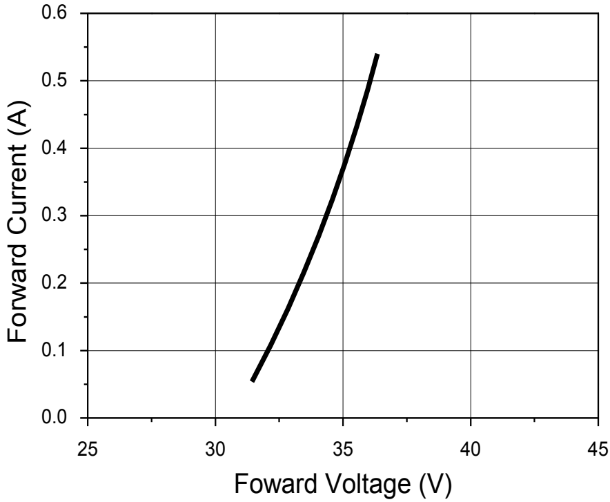
Fig 4. Forward Voltage vs. Forward Current, T_j=85^\circ\text{C}
